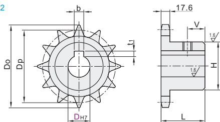
链条 ZVMN01/21
