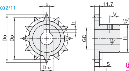
链轮 ZVL K02/11
